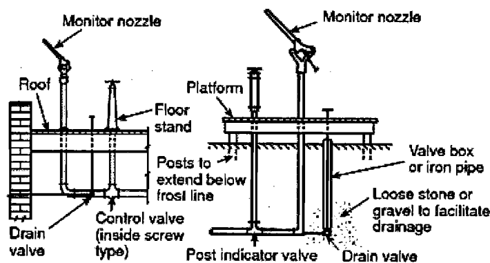
FIGURE A.3.3.22.1(b) Alternative Arrangement of Standard Monitor Nozzles.
